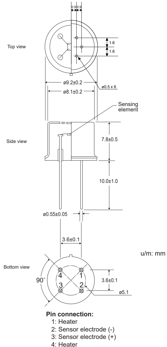
Fig. 3 - Sensor dimensions
