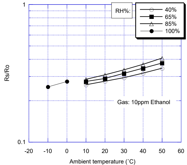
Fig. 7 - Temperature and humidity dependency ( R_s/R_o ) in 10ppm of ethanol
