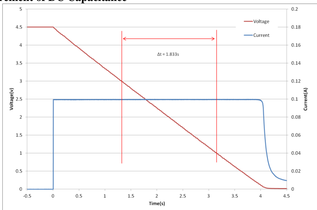
Fig 2: Measurement of DC Capacitance for a GA209
