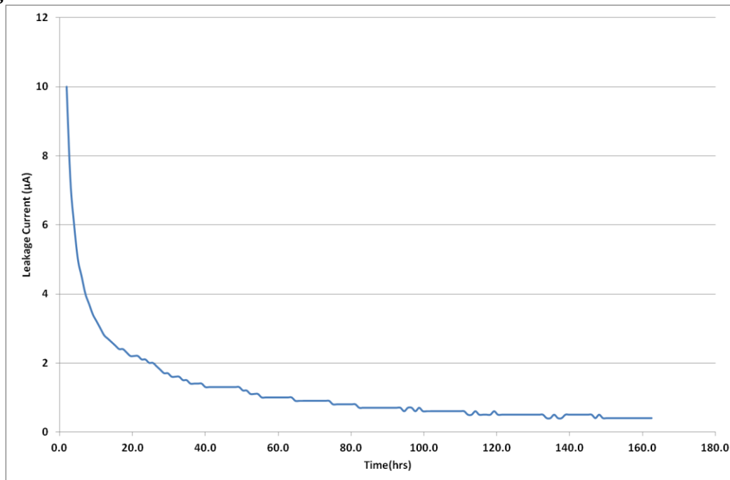
Fig 10: Leakage Current
