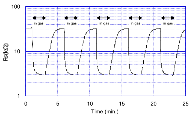
Fig. 10 - Repeatability
