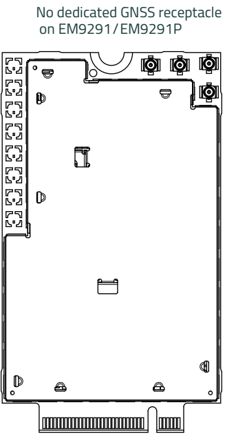
Top View — EM9291/EM9291P
