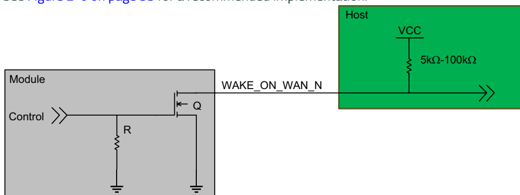
Figure 2-6: Recommended WAKE_ON_WAN_N Connection
