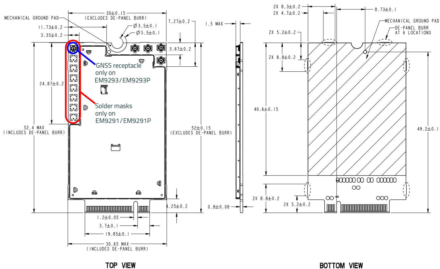
Figure 6-2: EM929X Dimensioned View of Mechanical Outline
