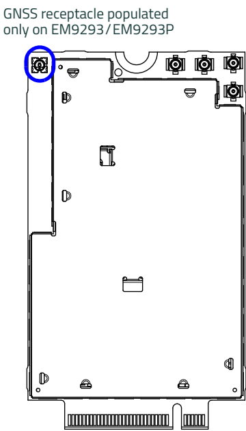
Bottom View — EM9291/EM9291P
