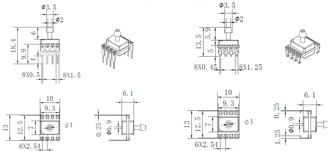
AN: Uniaxial Barbed Port
