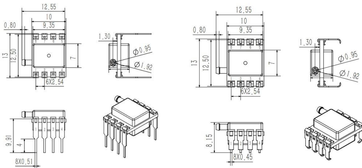
AN: Uniaxial Barbed Port
