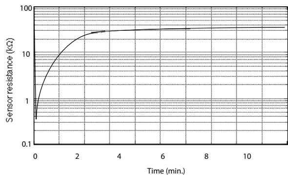
Fig. 12 - Initial action
