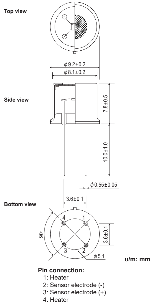
Fig. 3 - Sensor dimensions
