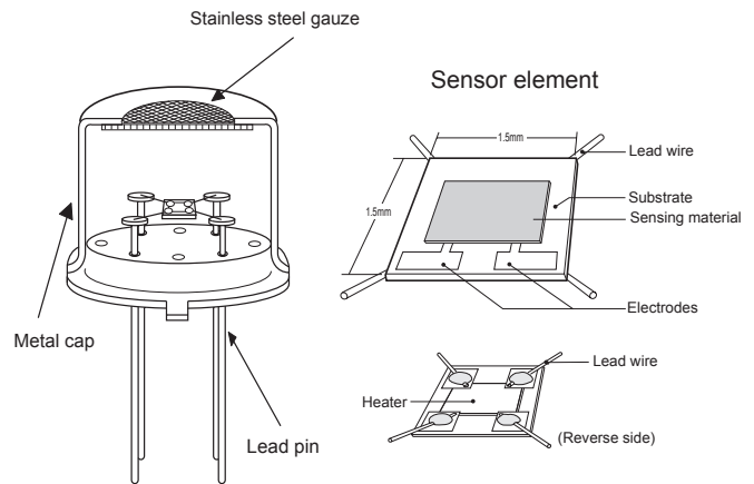
Fig. 1 - Sensor structure
