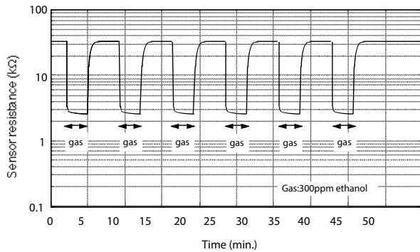
Fig. 11 - Repeatability
