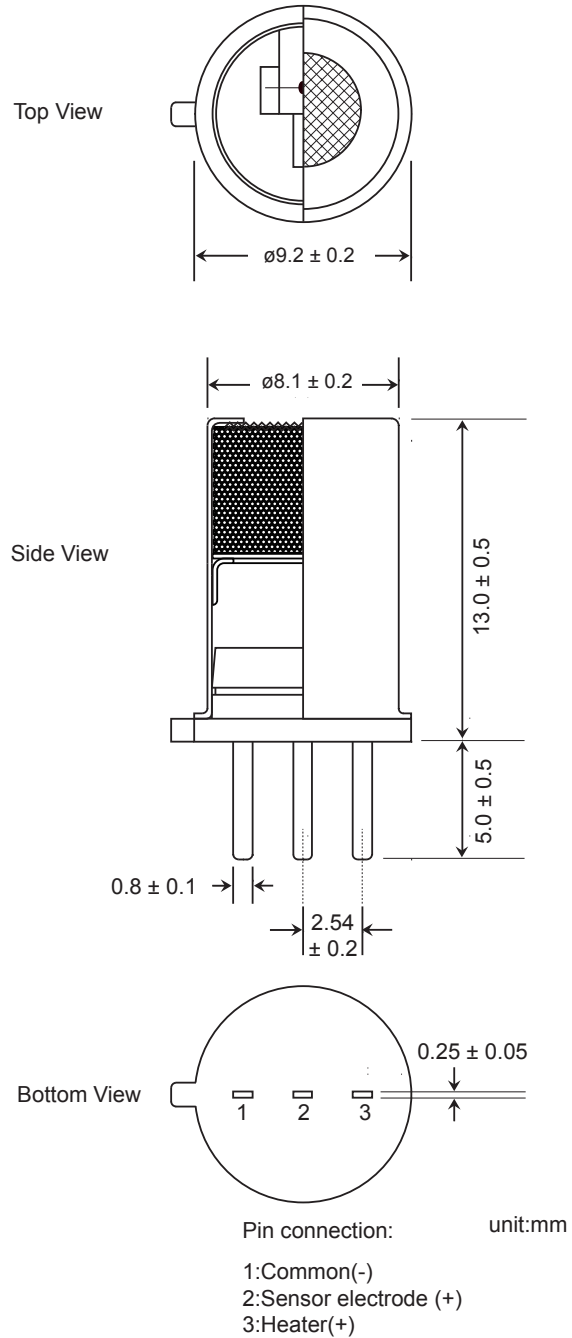
Figure 3 - Dimensions
