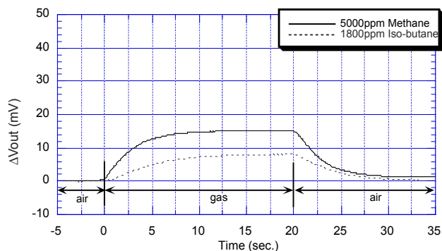
Fig. 8 - Gas response
