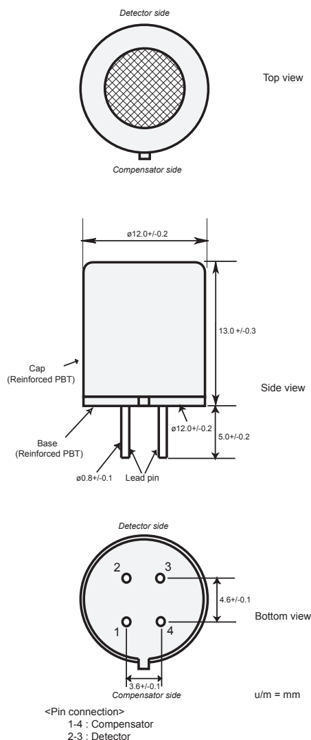
Fig. 3 - Sensor dimensions
