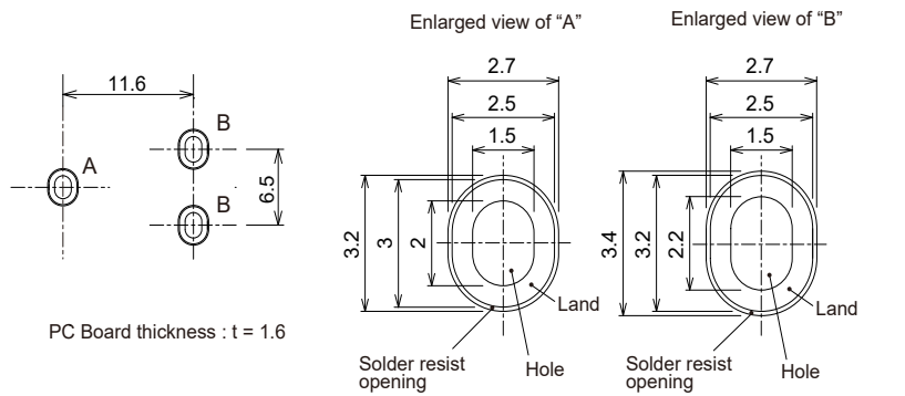
Figure 23 - Foot print example Unit : mm
