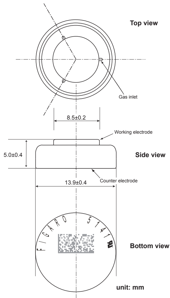
Figure 3 - Dimensions
