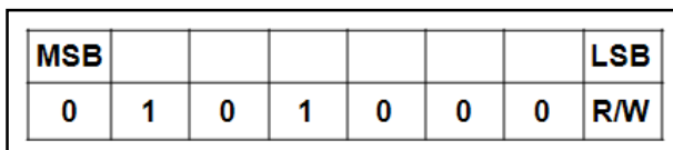
Figure 8 Address Byte
