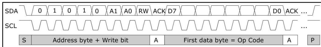
Figure 10 I²C principle sequence
