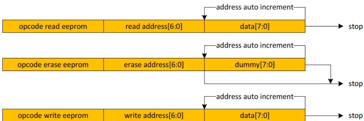
Figure 16 EEPROM communication
